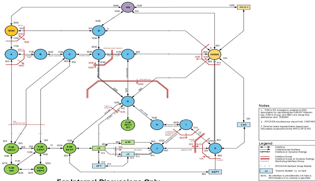
Draft Topology for 2021 IRM Study
