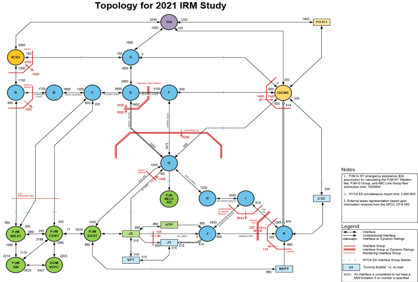
Figure A.11 2020 IRM Topology
