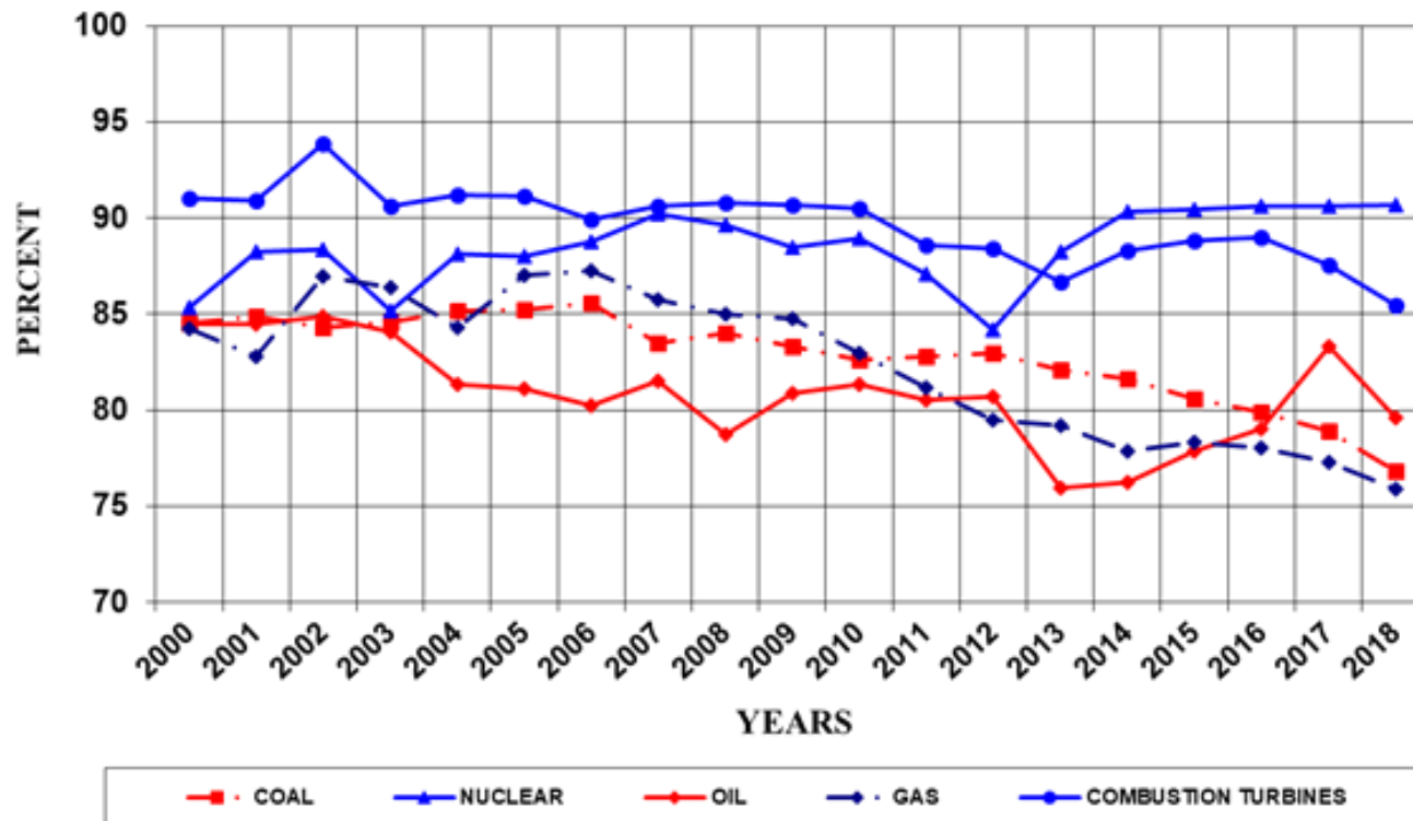
Figure A.7 NERC Annual Availability by Fuel
