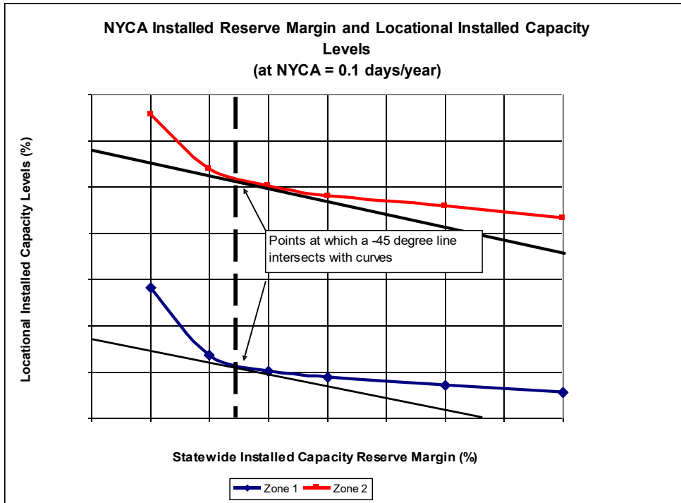
Figure 3-2: Unified Curve and IRM Anchor Point
