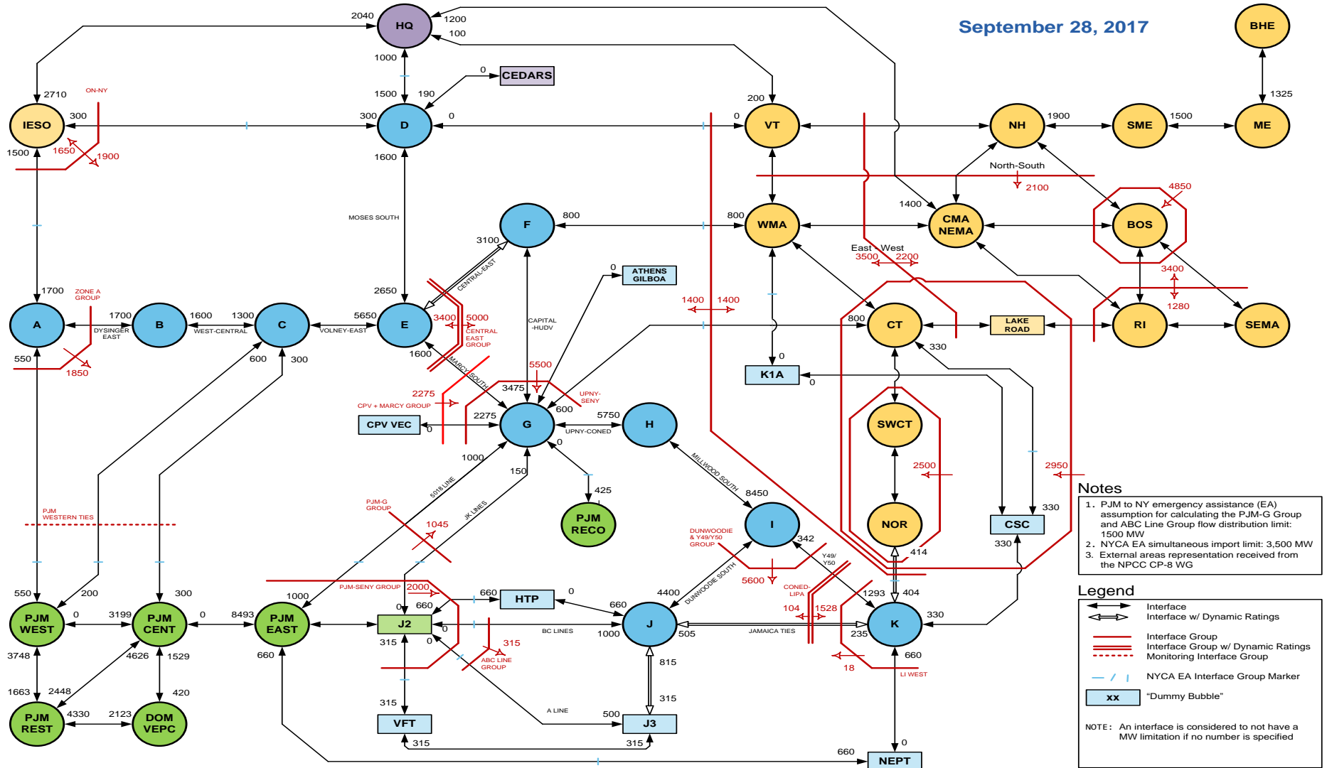
Figure A.12 2018 IRM Topology 2018 IRM Final Topology (Summer Ratings)
