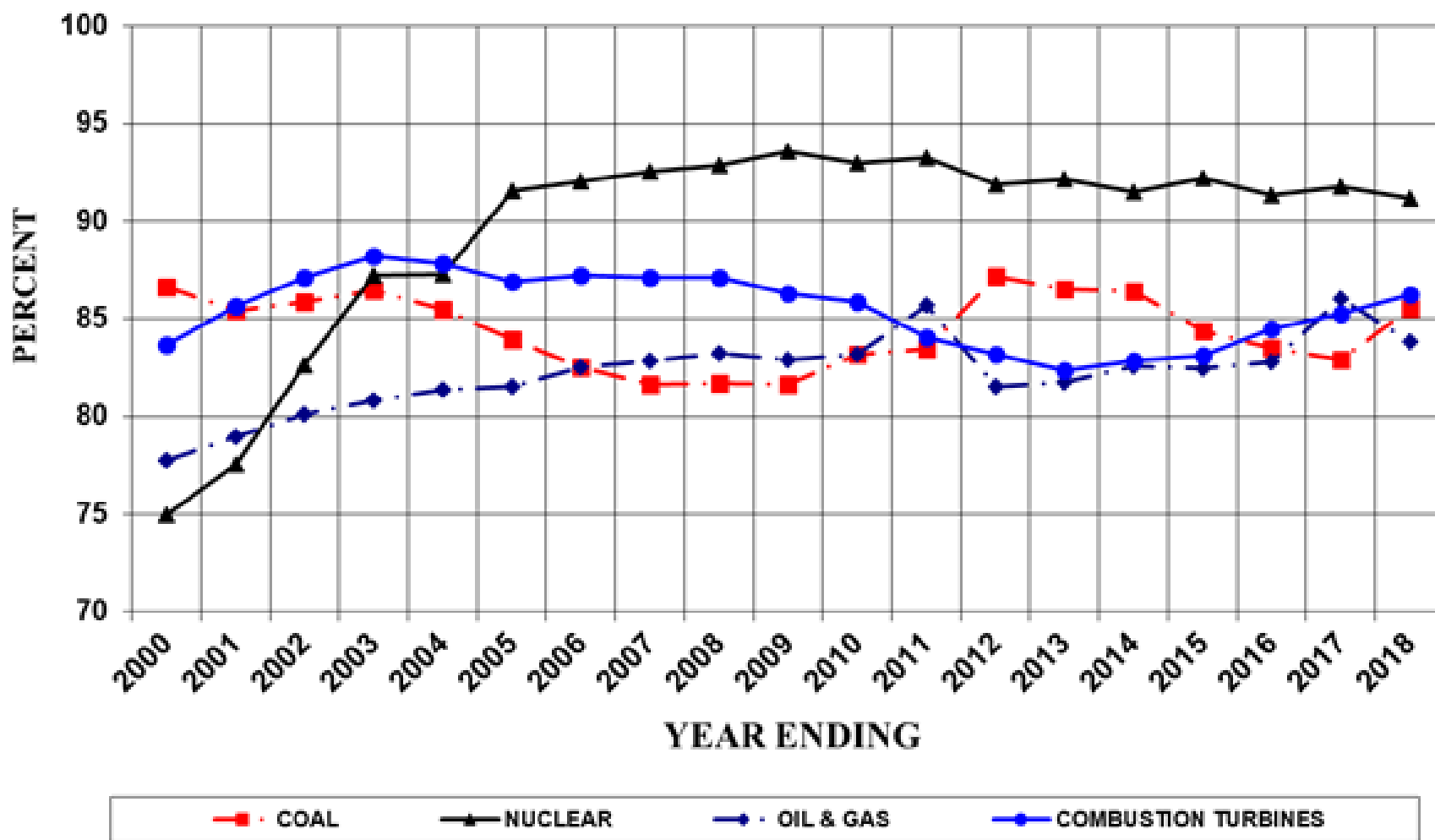
Figure A.6 NYCA Five-Year Availability by Fuel
