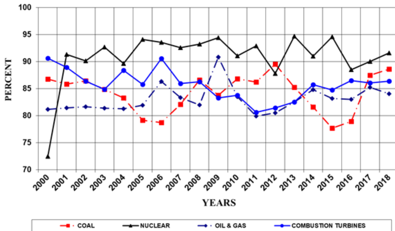
Figure A.5 NYCA Annual Availability by Fuel
