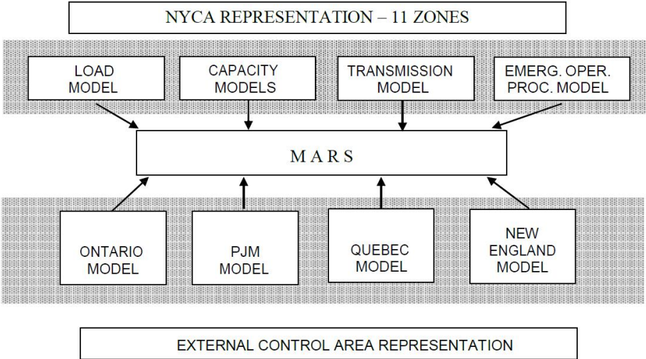
Figure A.1 NYCA ICAP Modeling
