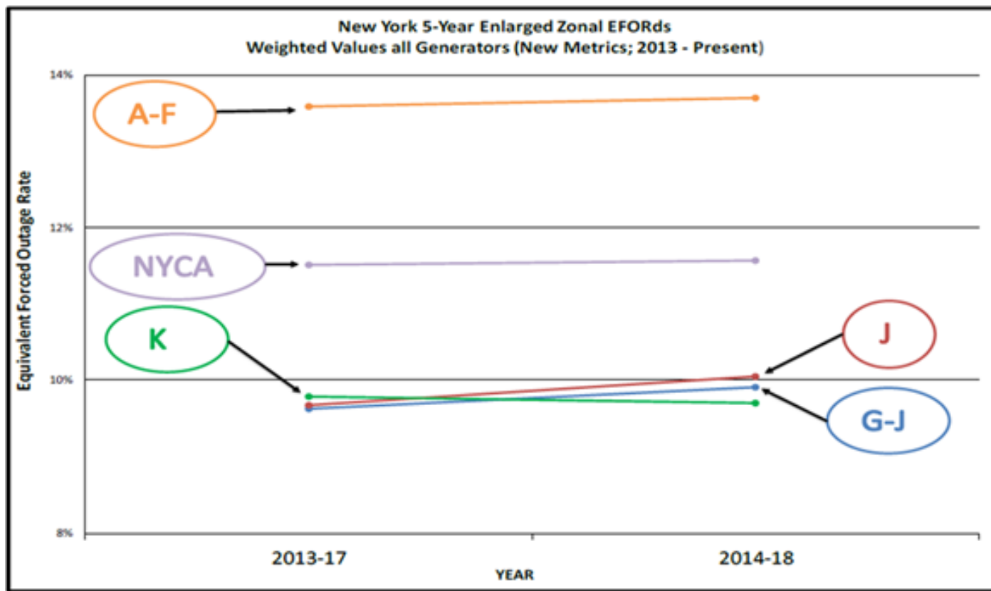
Figure A.4 Five-Year Zonal EFORDs
