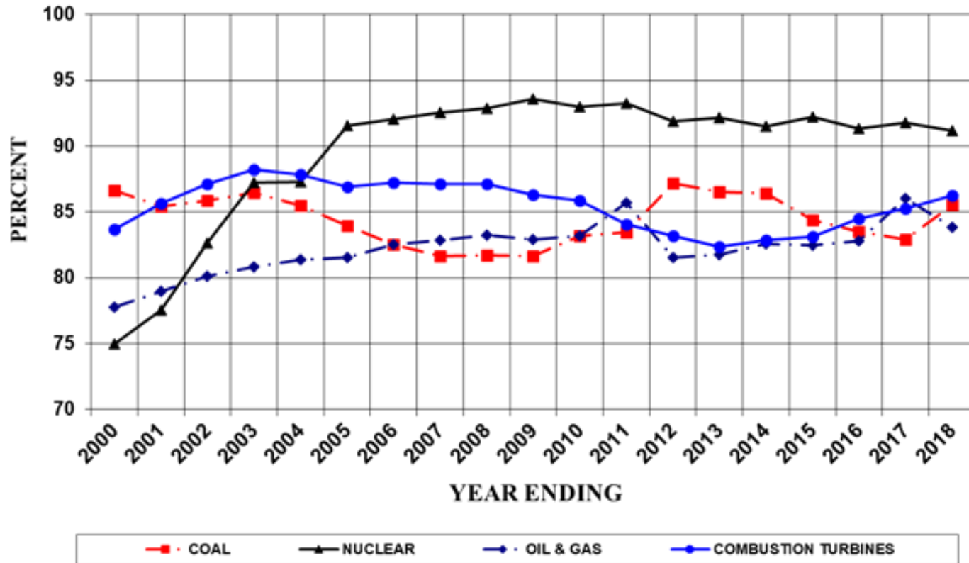
Figure A.6 NYCA Five-Year Availability by Fuel
