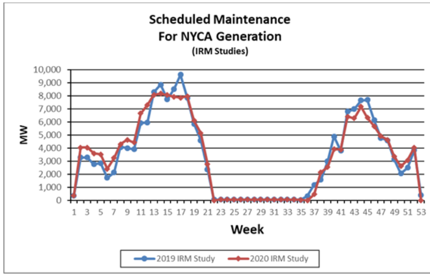
Figure A.10 Scheduled Maintenance
