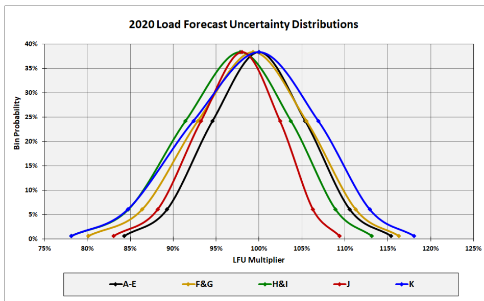
Figure A.2 LFU Distributions
