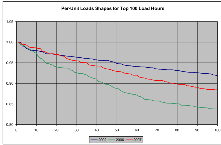
Figure A.3 Per Unit Load Shapes
