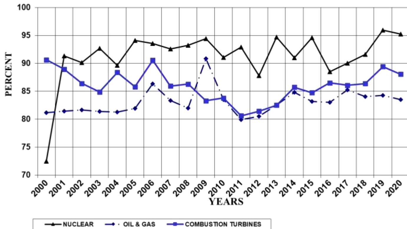
Figure A.6 NYCA Annual Availability by Fuel
