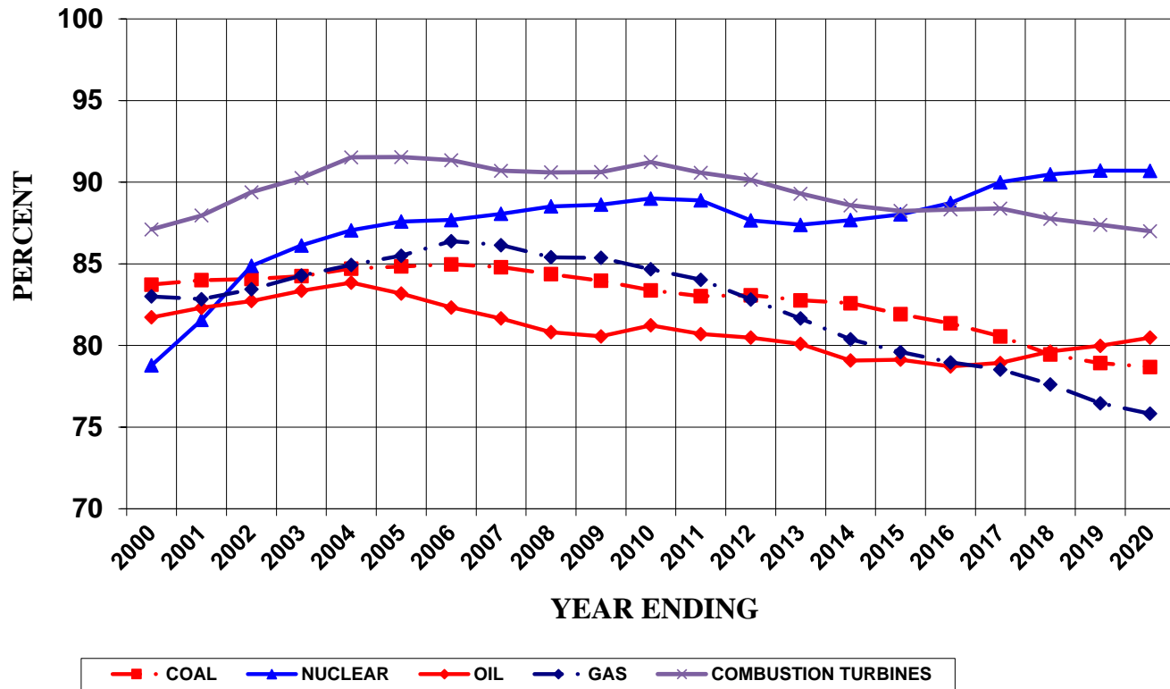
Figure A.9 NERC Five-Year Availability by Fuel
