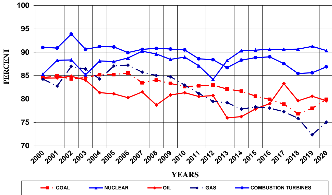
Figure A.8 NERC Annual Availability by Fuel
