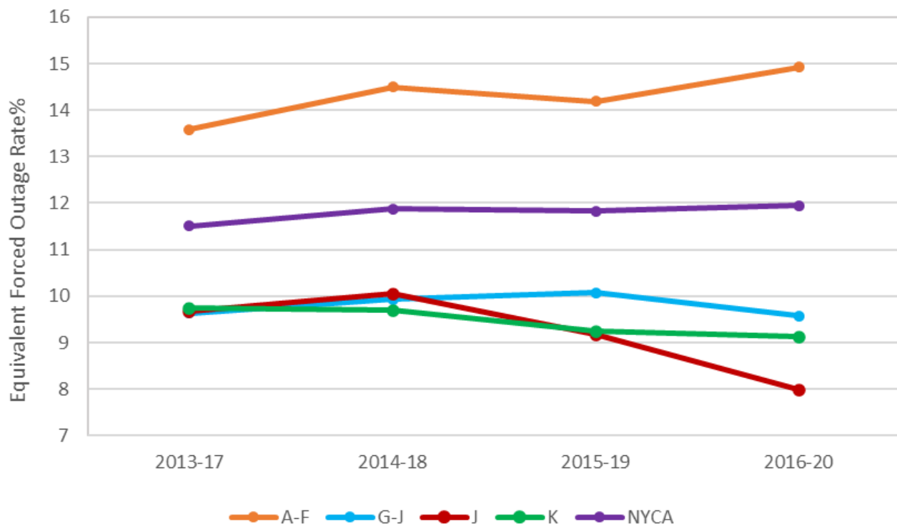
Figure A.5 Five-Year Zonal EFORDs
