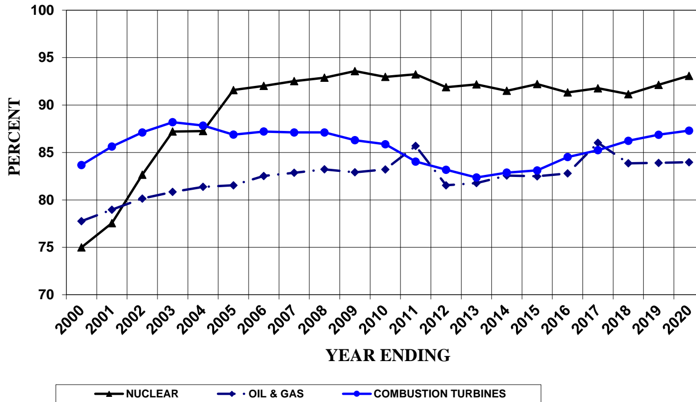
Figure A.7 NYCA Five-Year Availability by Fuel
