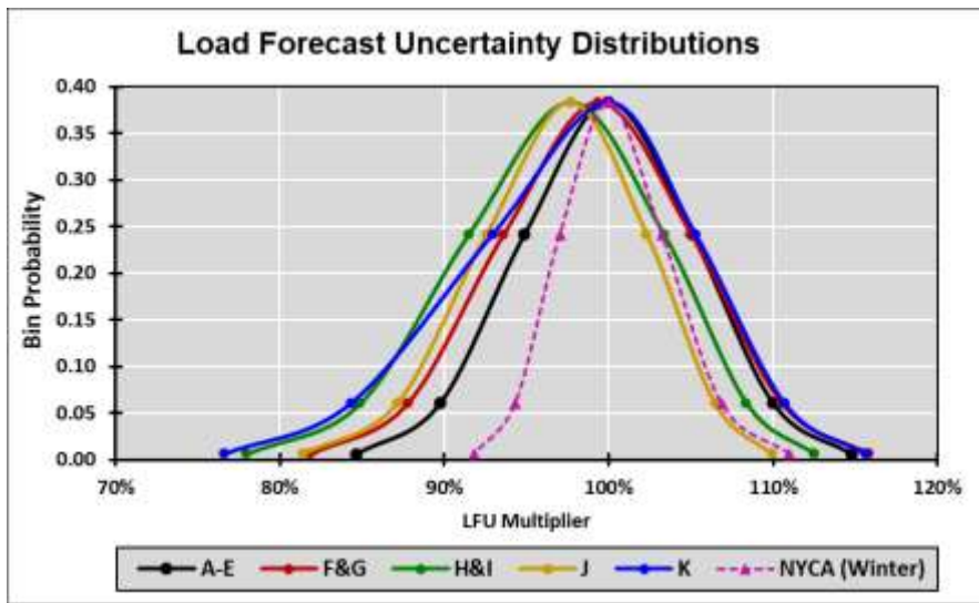
Figure A.4 LFU Distributions
