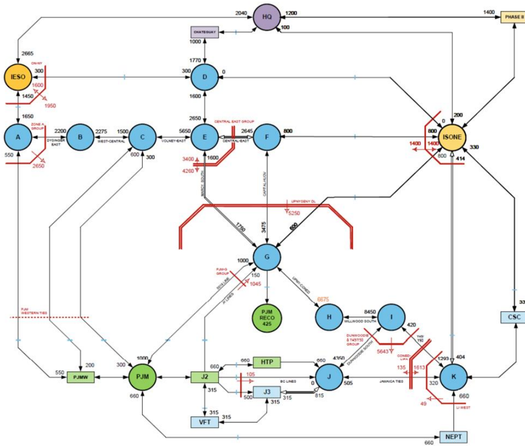
Figure A.10 2023 IRM Topology
