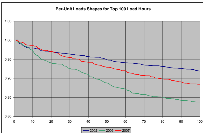
Figure A.3 Per Unit Load Shapes
