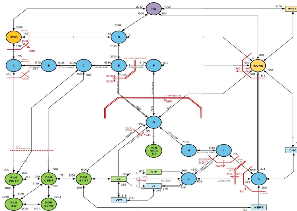
Draft Topology for 2021 IRM Study
